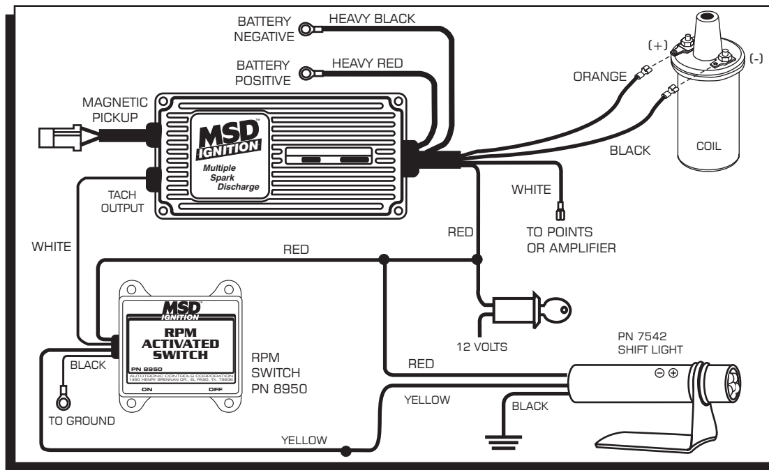
Figure 2 Connecting with an RPM Activated Switch.
