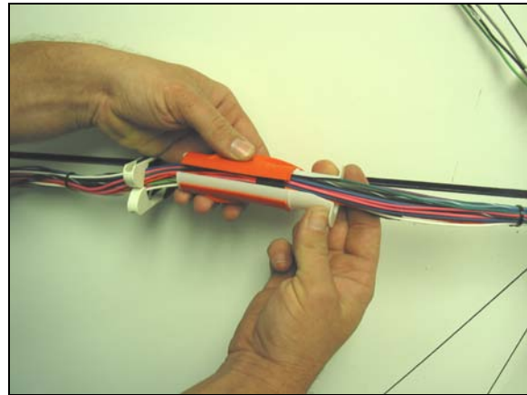
The tool is then closed around the wire
