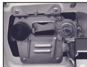
Window Regulator
