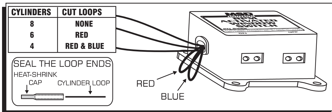
Figure 2 Cylinder Select Loops.
