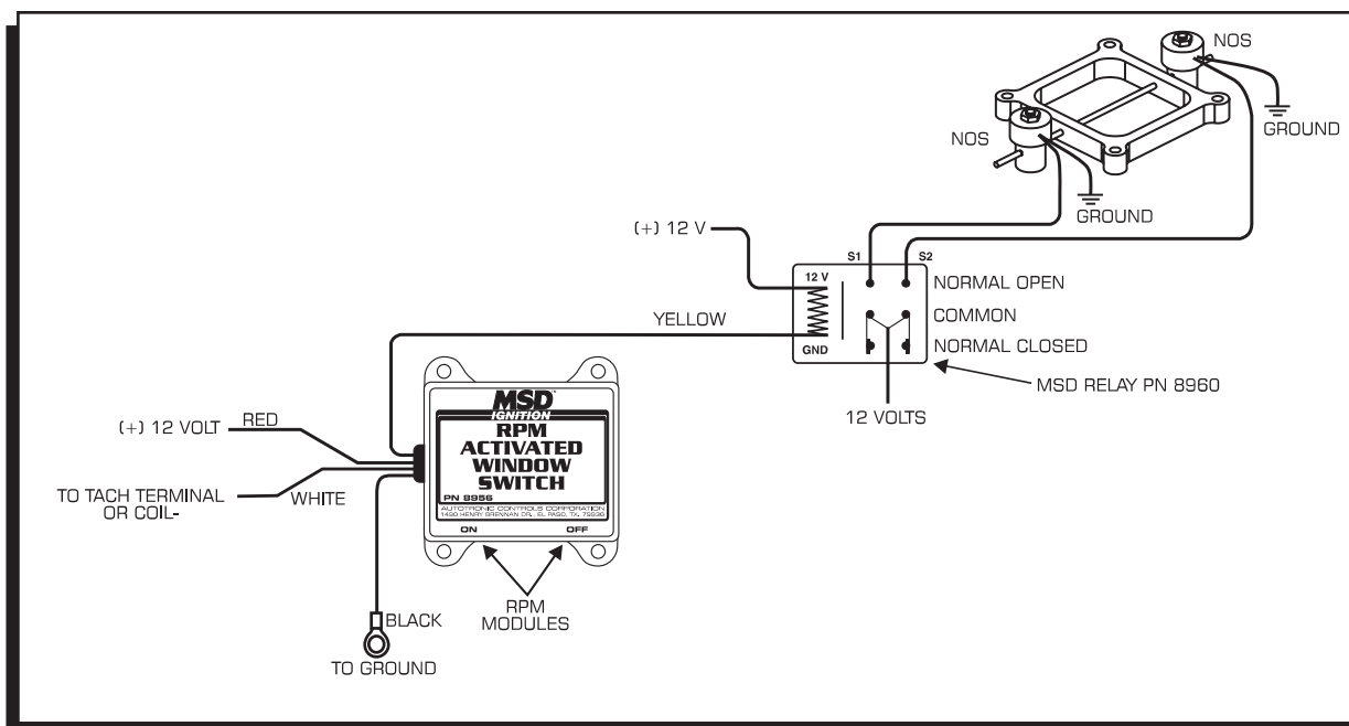
Figure 5 Wiring with an MSD Relay.
