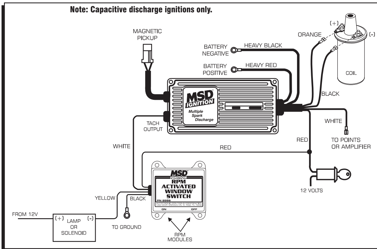
Figure 4 Wiring to an MSD Ignition Control.
