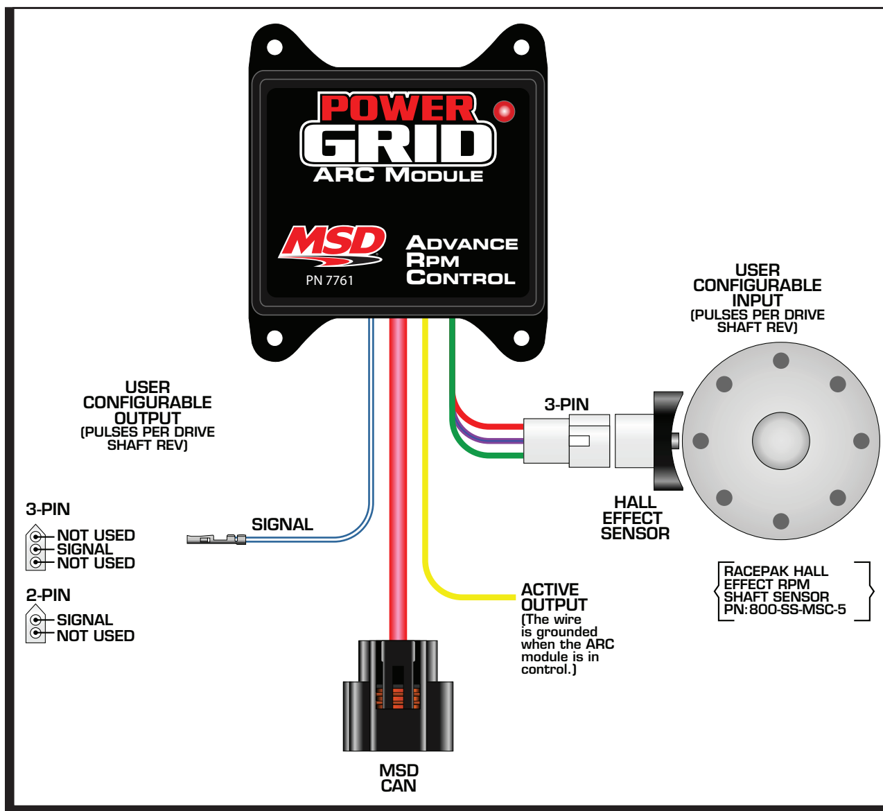
Figure 2 Wiring.
