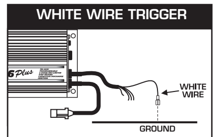
Figure 11 Checking for Spark with the White Wire.
