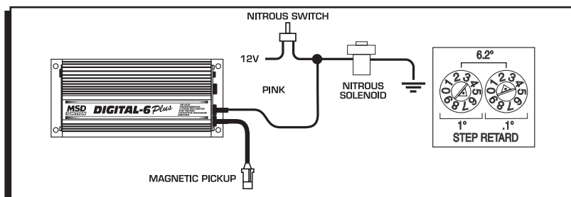
Figure 6 Wiring the Retard Stage.
