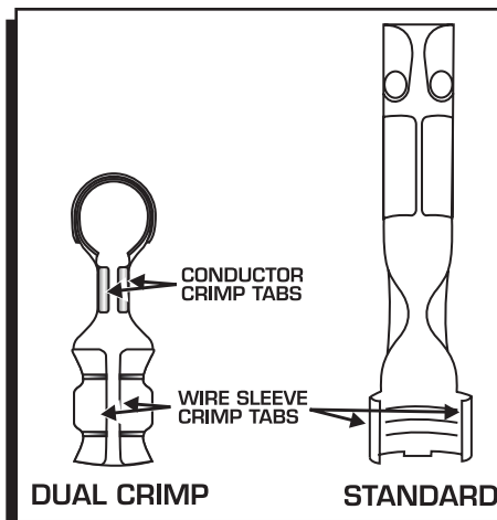
Figure 1 Identifying the Different Style Terminals.
