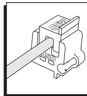
Figure 6 Aligning the Terminal in Tool.
