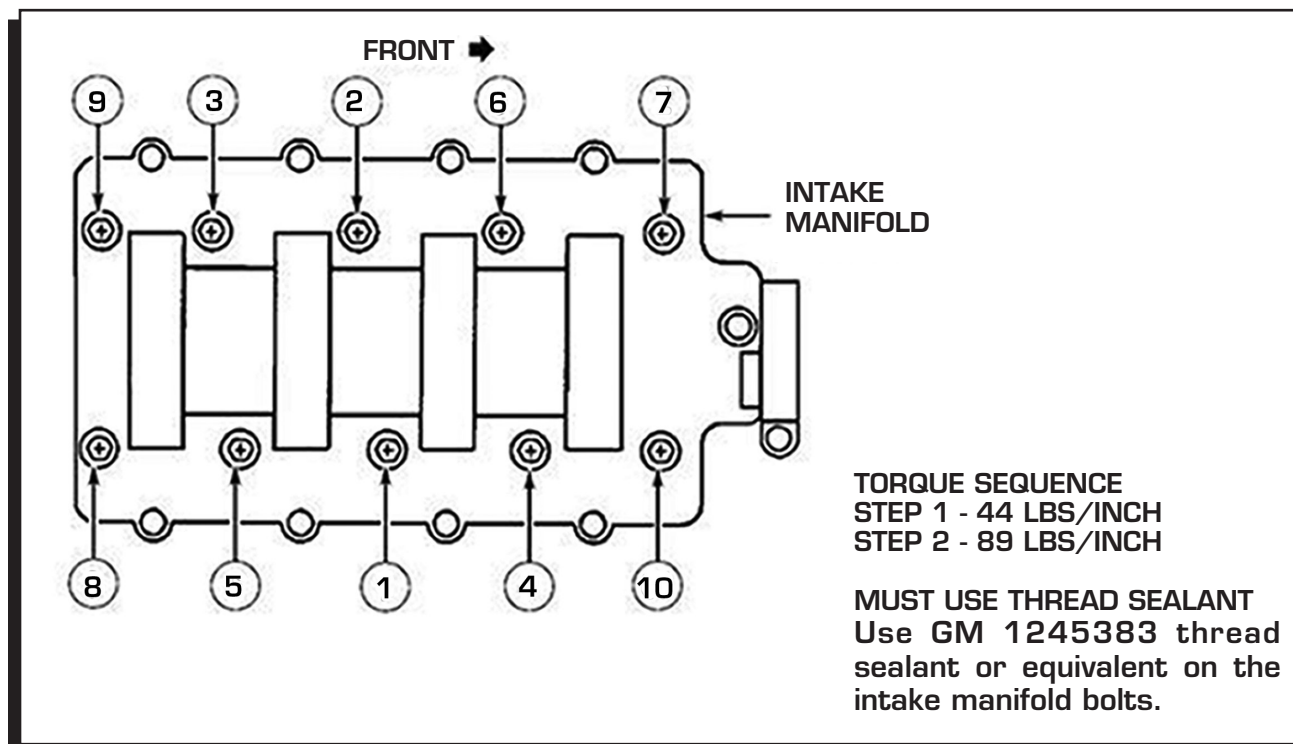
Figure 2 Intake Manifold Bolt Tightening Sequence.
