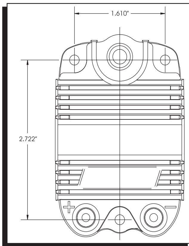
Figure 1 Mounting Template.
