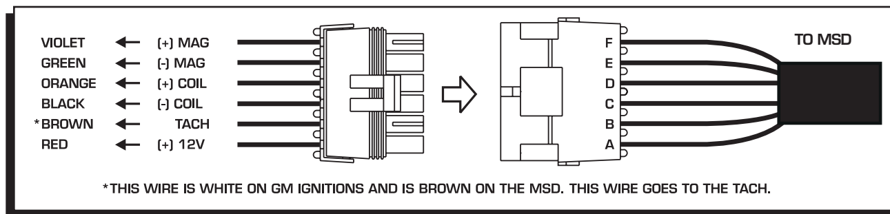
Figure 1 The Color, Function and Position of Each Wire.
