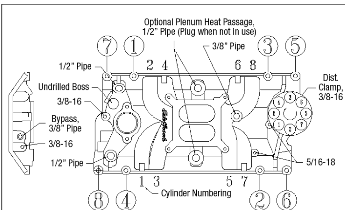
Figure 4 - Intake Manifold Tightening Sequence
