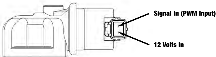
Figure 3 - Throttle Position Sensor (TPS)
