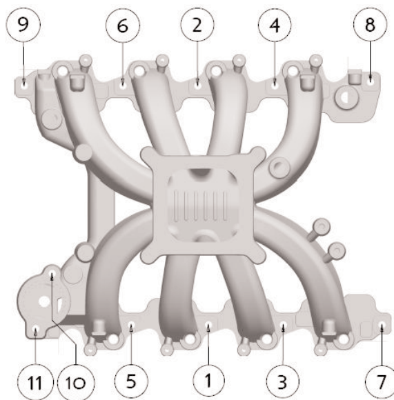
Figure 1 - Torque Sequence Torque manifold bolts to 15-20 ft/lbs.
