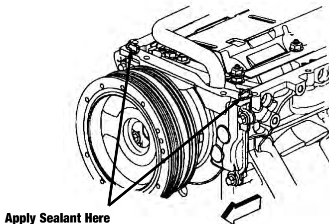
Figure 3 - Sealant Locations
