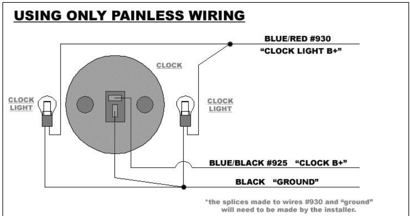
Figure 7-29B Clock Wiring
