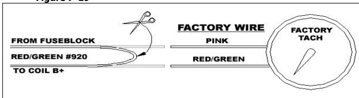
Figure 7-19 Factory Tach. Connections
