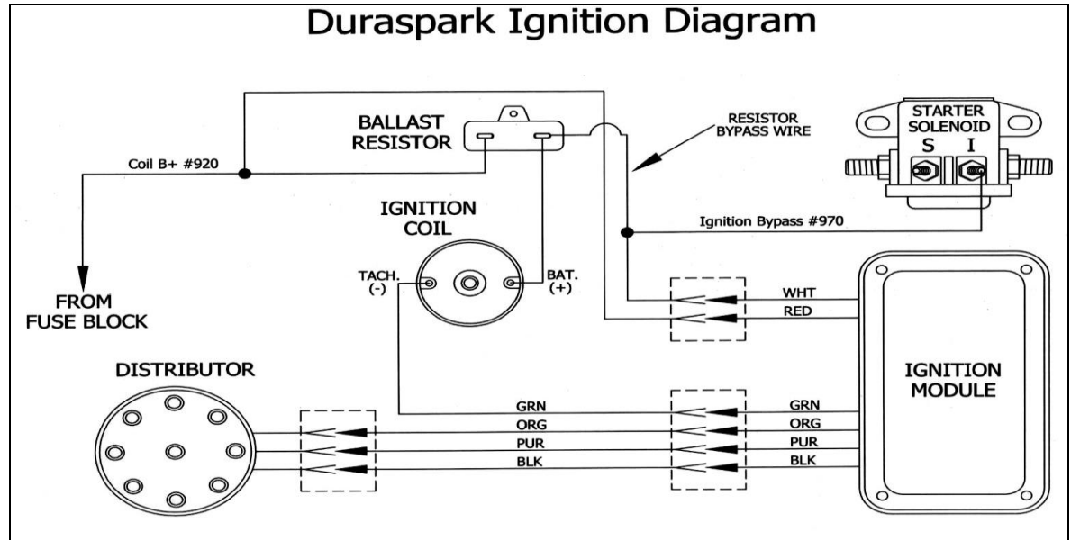
Figure 7-6 Ford Duraspark II Systems (Ford Electronic Ignition)
