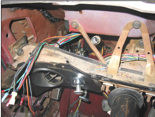
Figure 6-9 Interior Section Routing
