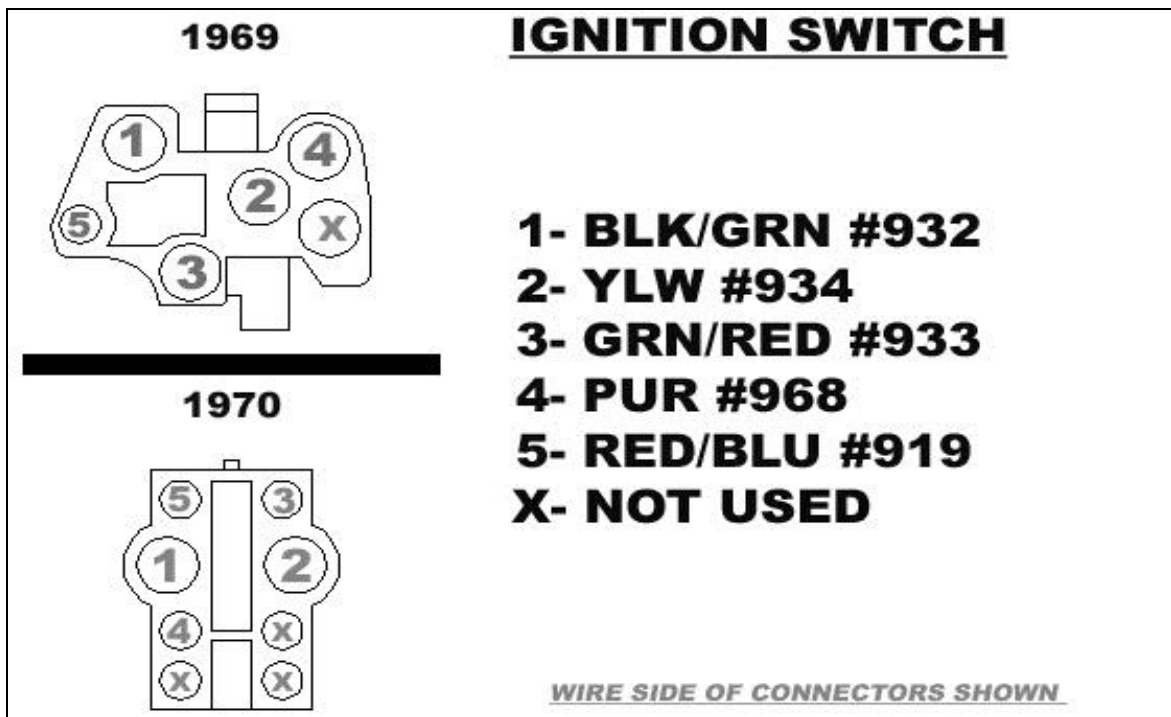
Figure 7-20C Ignition Switch Connection
