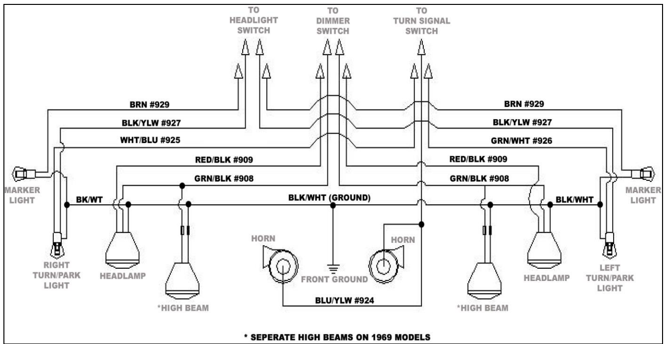
Figure 7-11 Headlight Section Connections
