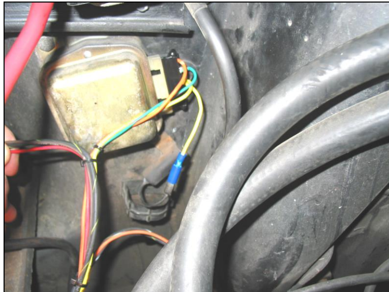
Figure 7-2 Regulator Connections
