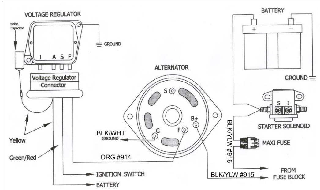
Figure 7-1 Alternator/Regulator Connections
