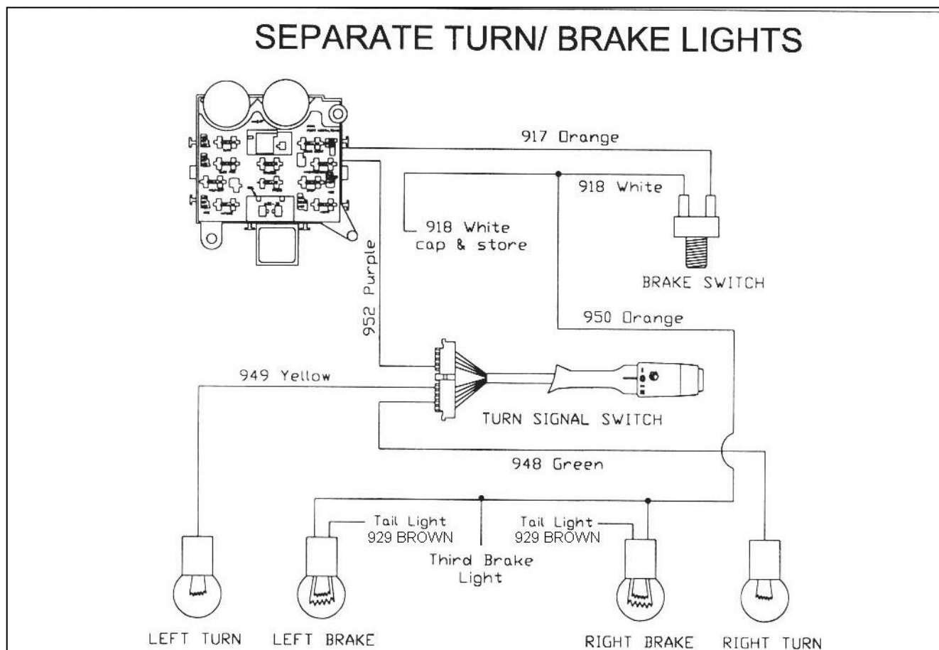
Figure 15-2 Separate Turn/Brake Lights
