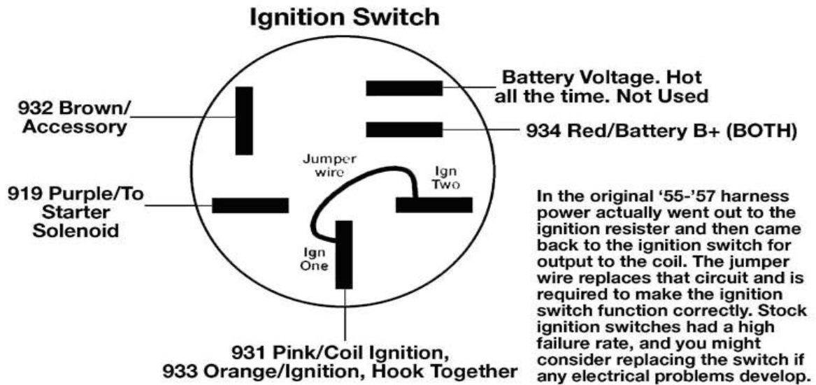
Figure 9.1 1955-1957 Chevrolet Ignition Switch
