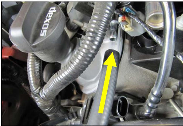
10. Slide the 3/8"Breather Hose onto the steel crankcase breather tube on the valve cover. Refer to step #3.
