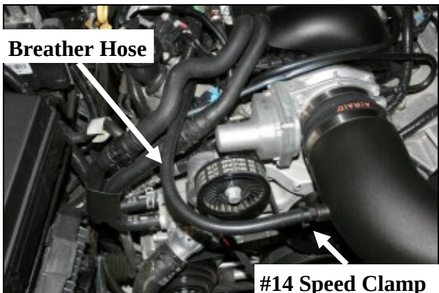
16. Install the 3/8 " barbed fitting (#13) into the Airaid Intake Tube. Next install the 3/8"x18" breather hose between the barbed fitting and the steel crankcase breather tube on the rocker cover. Refer to step #2. Install one #14 speed clamp (#12) over the breather hose at the barbed fitting as shown.
