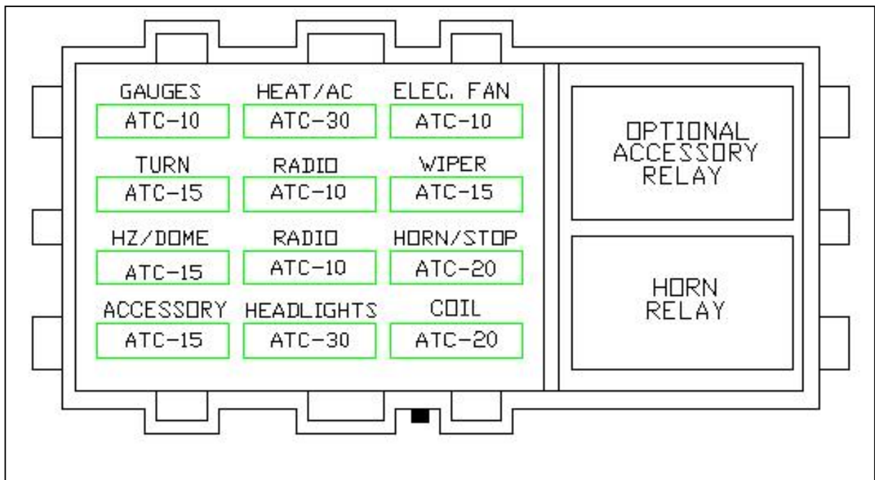
Figure 9.1 Fuse Requirements
