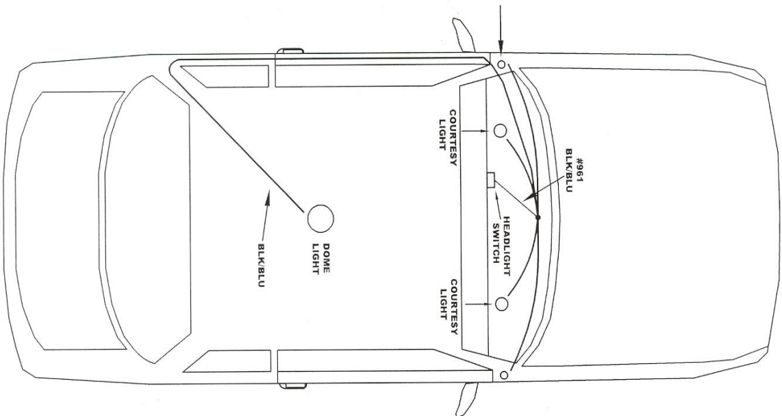
Figure 8-2 Interior Lighting
