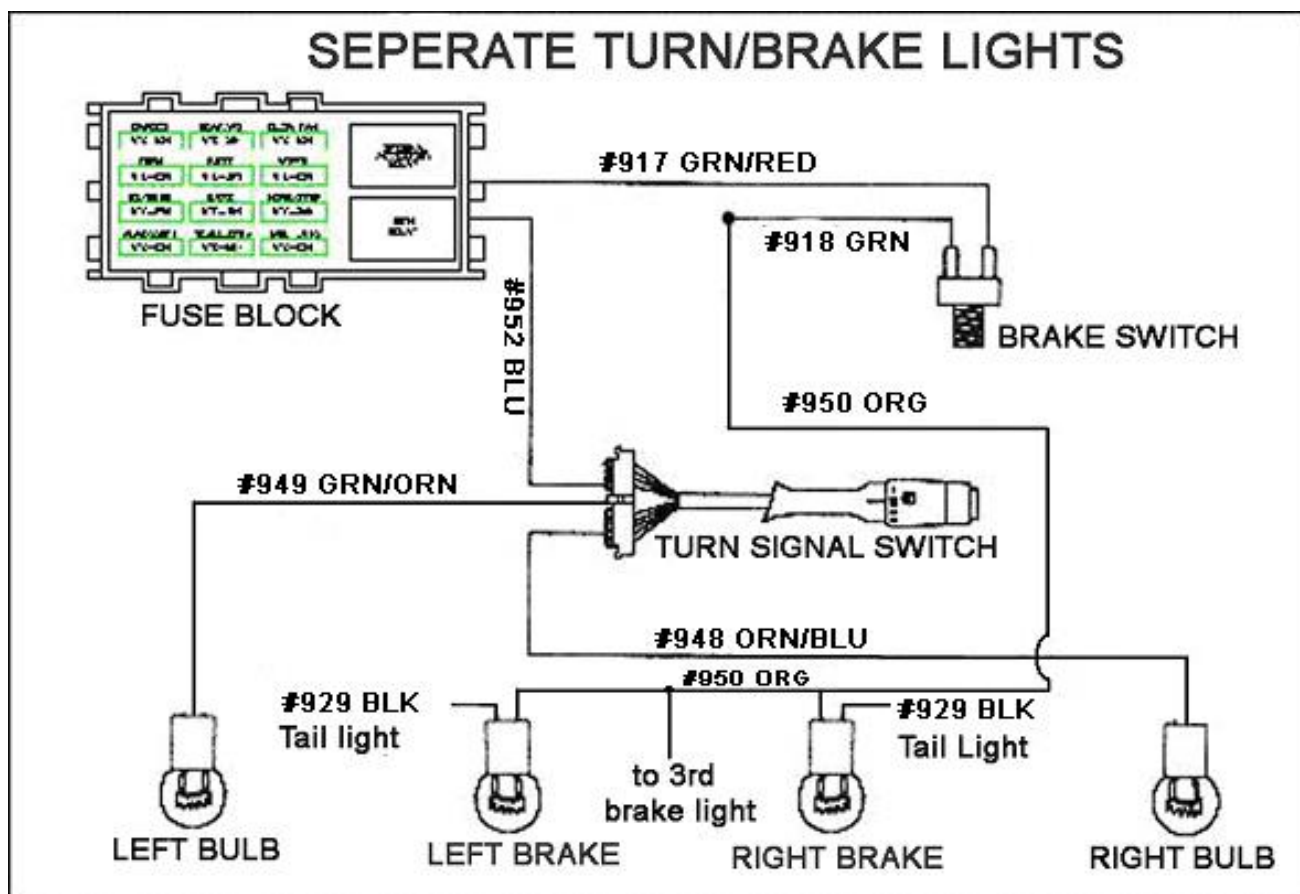
Figure 8-7B Separate Turn/Brake Lights
